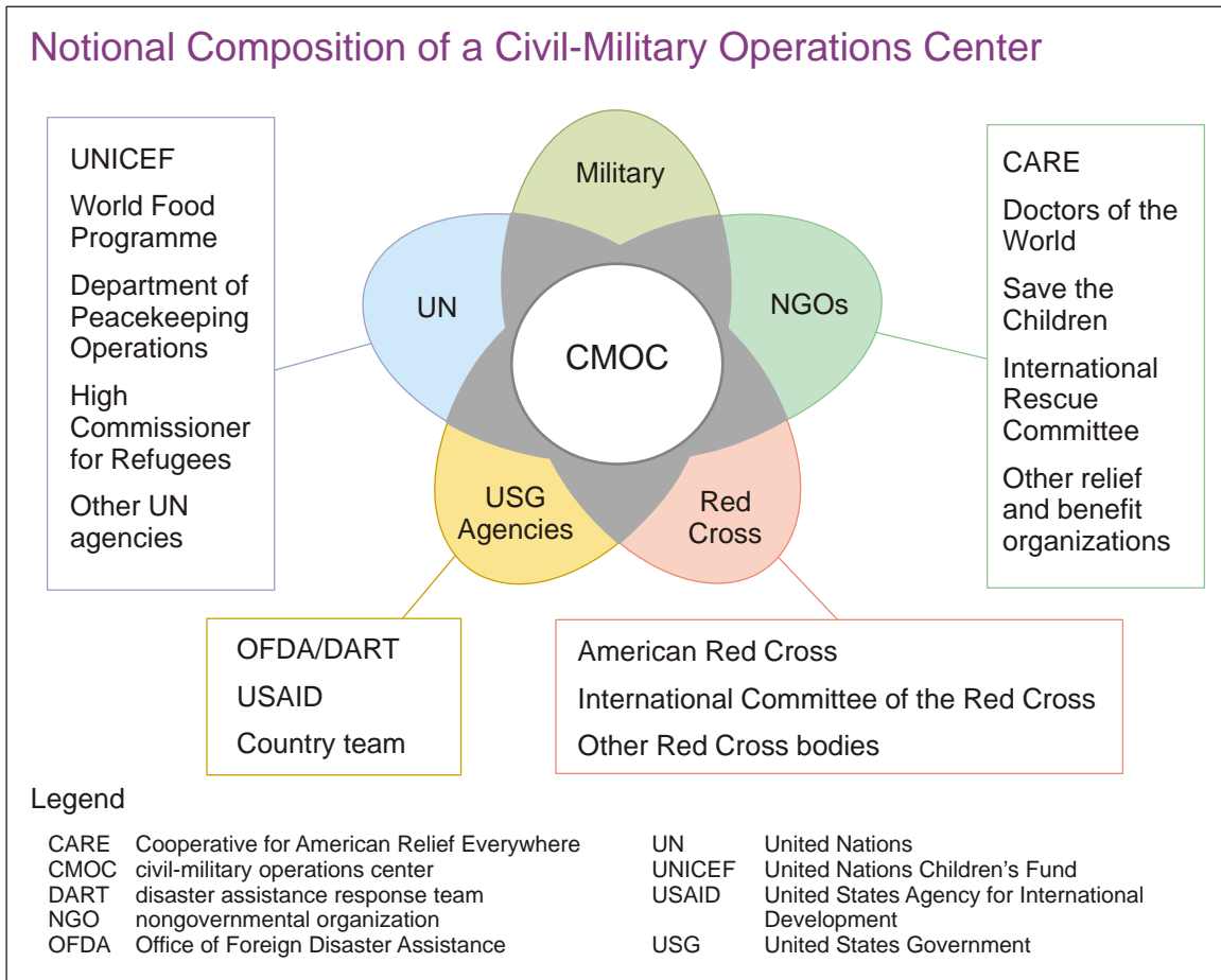
Figure II-5. Notional Composition of a Civil-Military Operations Center
